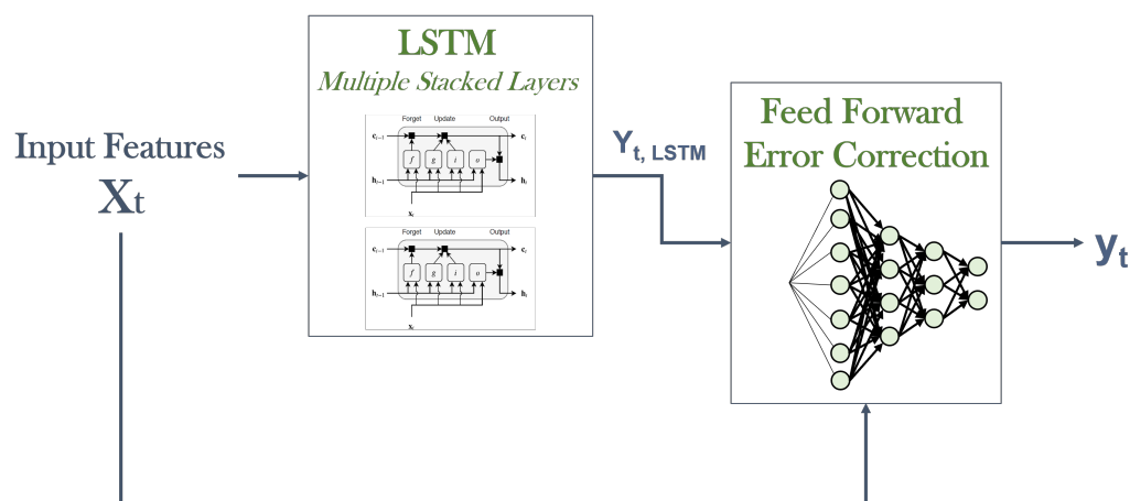
Figure 6. LSTM with Feed-Forward Error Correction architecture.
