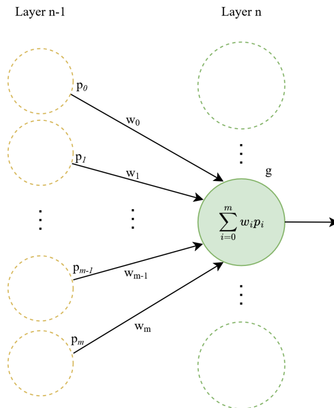
Figure 3. An artificial neuron architecture.
