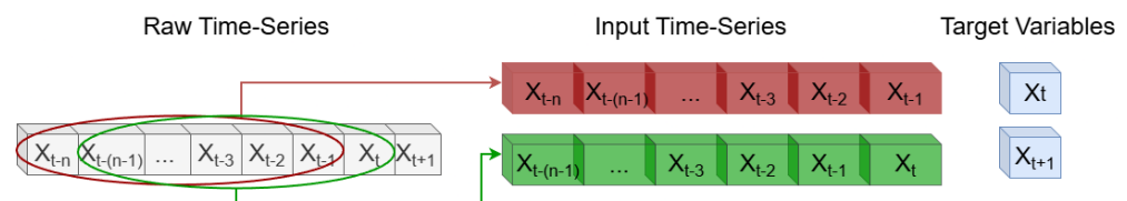
Figure 2. Time Step Shifting Mechanism for training/test time series creation.
