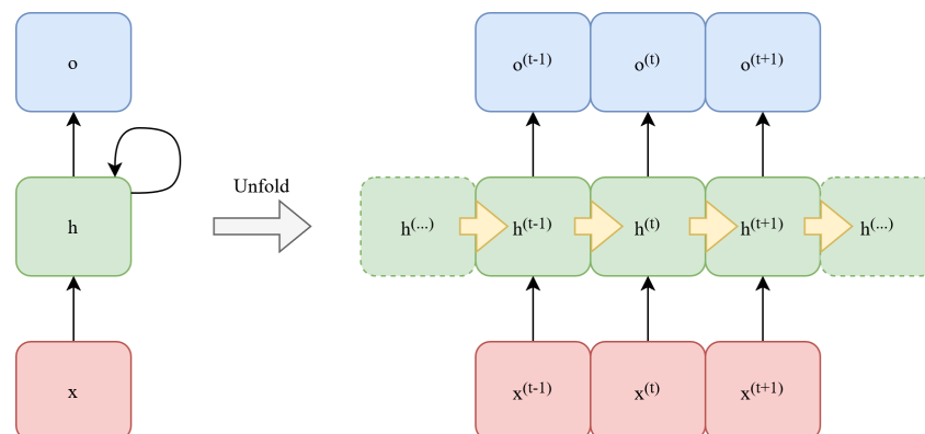
Figure 4. A simple RNN neuron (left) and its unrolled form over sequential time steps (right).
