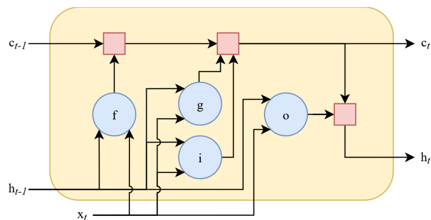
Figure 5. The architecture of an LSTM neuron.
