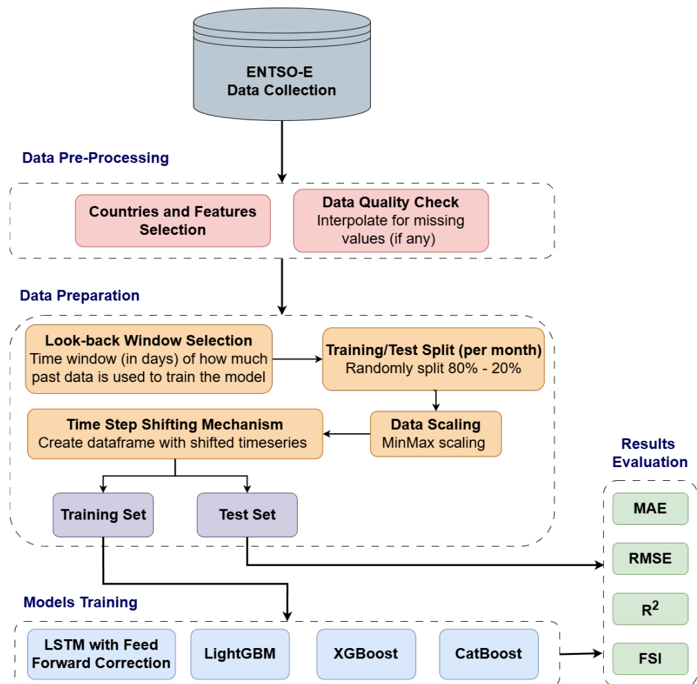
Figure 1. Proposed methodology for Day-Ahead Market price forecasting under different look-back windows and a monthly training/test set split.
