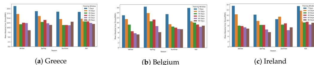
Figure 8. Seasonal MAE for different training windows across Greece, Belgium, and Ireland.
